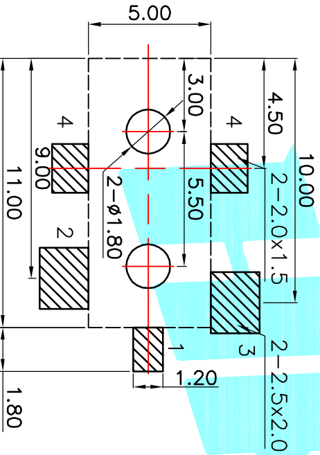
P.C.B LAYOUT(Copper-side view)
