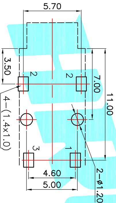
P.C.B LAYOUT(copper-sided view)
