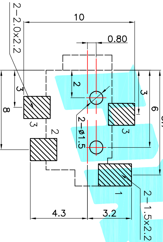
P.C.B LAYOUT(Copper-side view)
